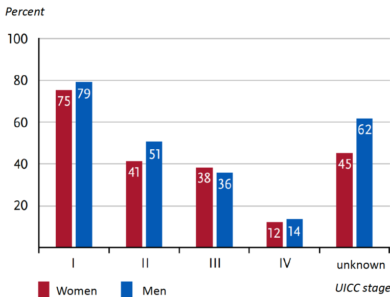
Figure 5: Relative 5-year survival by UICC stage (7th and 8th edition TNM) and gender, ICD-10 C67, Germany 2019-2020
